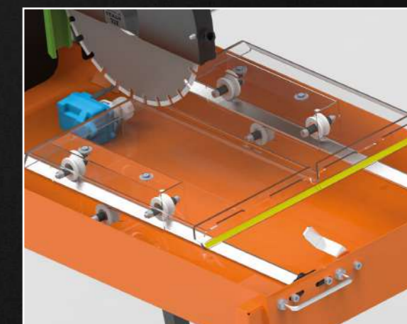
Working table sliding on 6 nylon wheels: in top 4 pulleys with 8 ball bearings; below 2 pulleys on 4 bushes in stainless steel. Higher precision and stability
